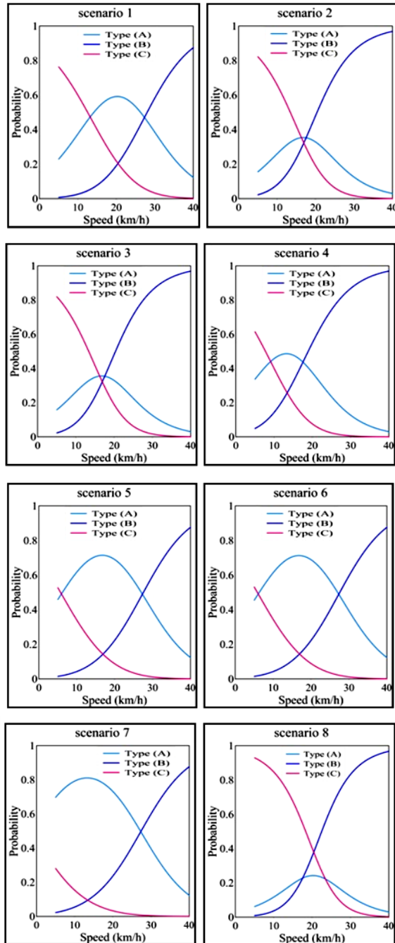
Figure 8. The choice probability of the speed profiles dependent on the initial speed and the exposure type
