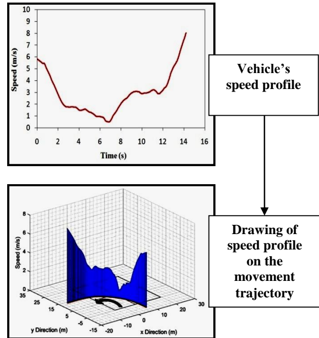
Figure 2. Process of drawing speed profiles
